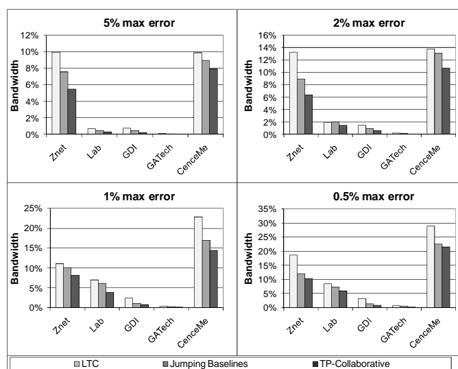
Figure 52 Bandwidth for lossy algorithms, all datasets
