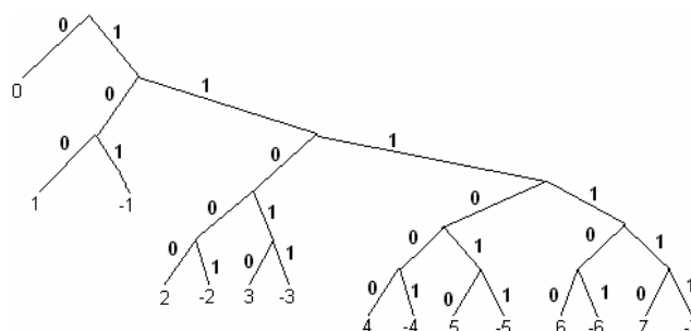
Figure 19 Huffman tree
