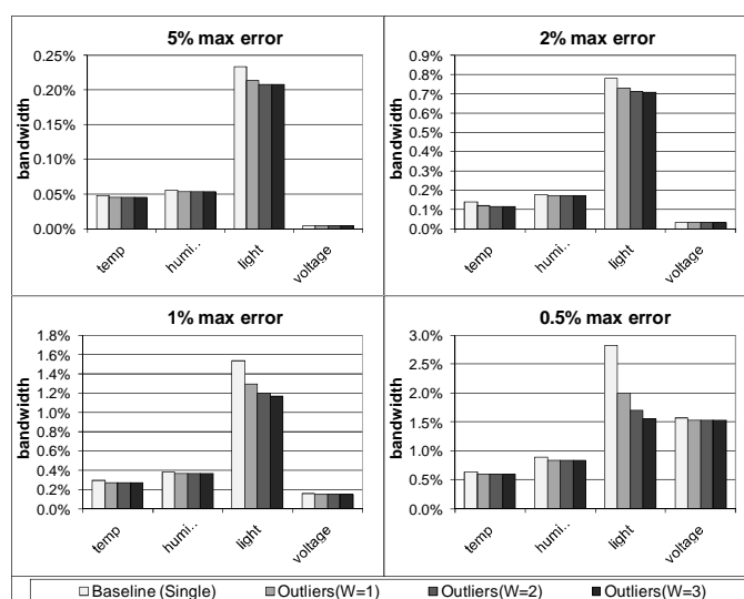
Figure 45 Bandwidth savings with outlier detection
