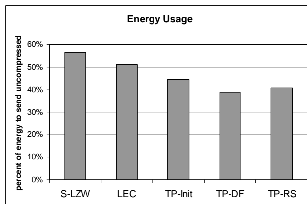
Figure 9 Energy usage
