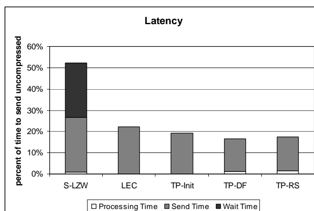
Figure 8 Latency
