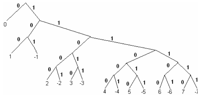
Figure 1 Huffman tree
