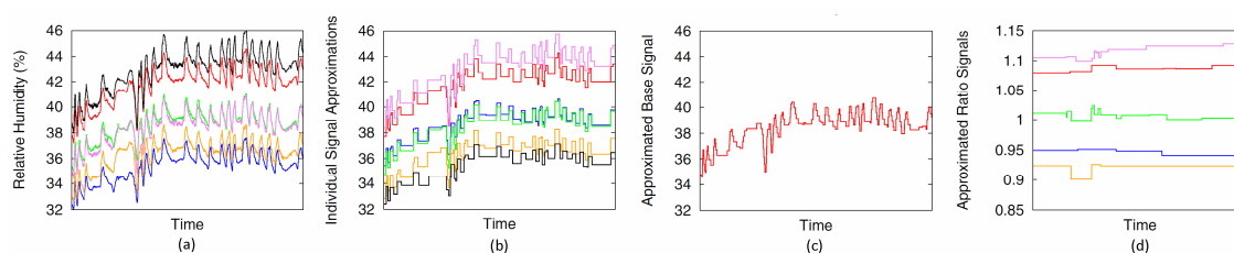
Figure 20 Gamps example
