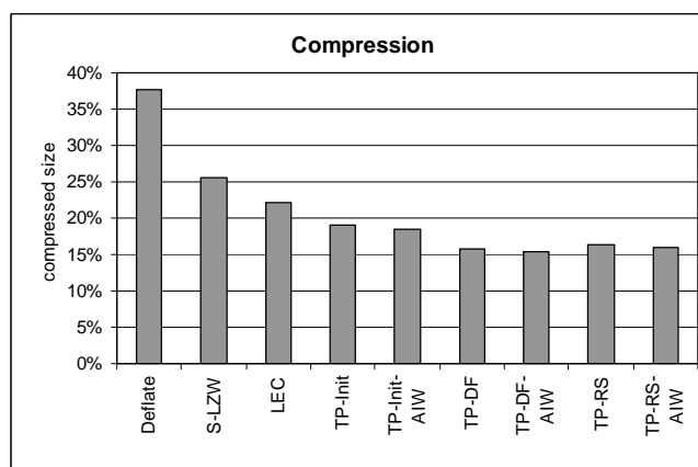
Figure 6 Compression summary
