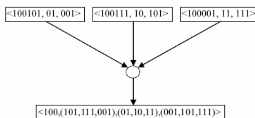
Figure 21 Pipelined compression
